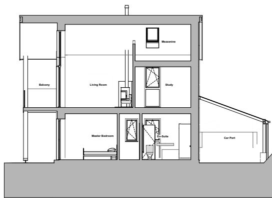
S-01 Building Section 1:100
