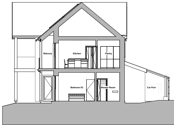
S-04 Building Section 1:100
