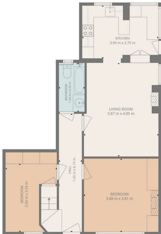
1ST FLOOR
