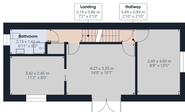
Floor 1 Building 1
