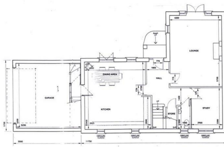
GROUND FLOOR LEVEL SCALE 1:50
