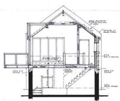
CROSS SECTION A-A
