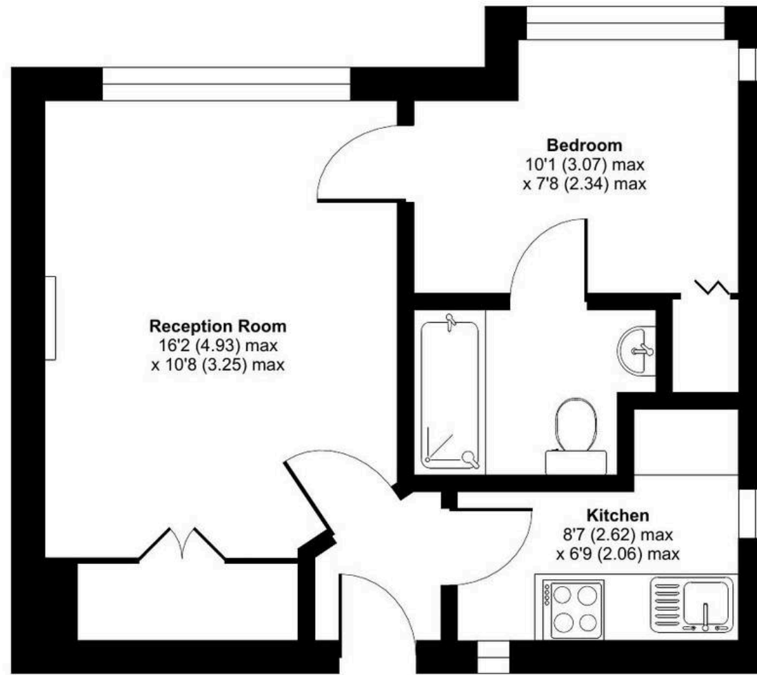
FIRST FLOOR
