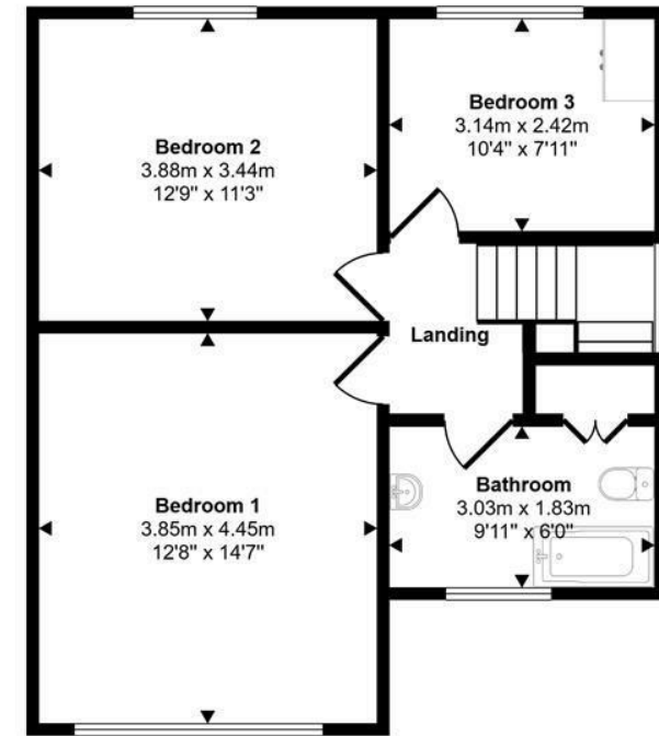
First Floor Approx 52 sq m / 561 sq ft
