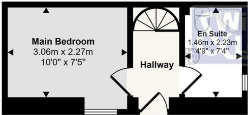
Ground Floor Approx 15 sq m / 165 sq ft
