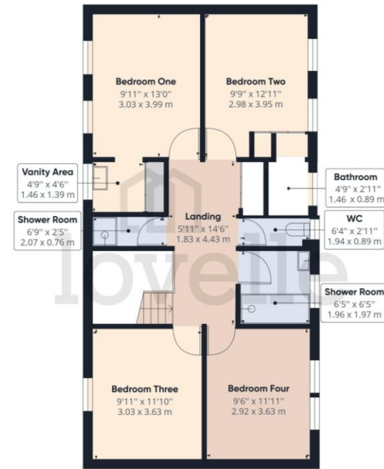
Floor 1 Building 1
