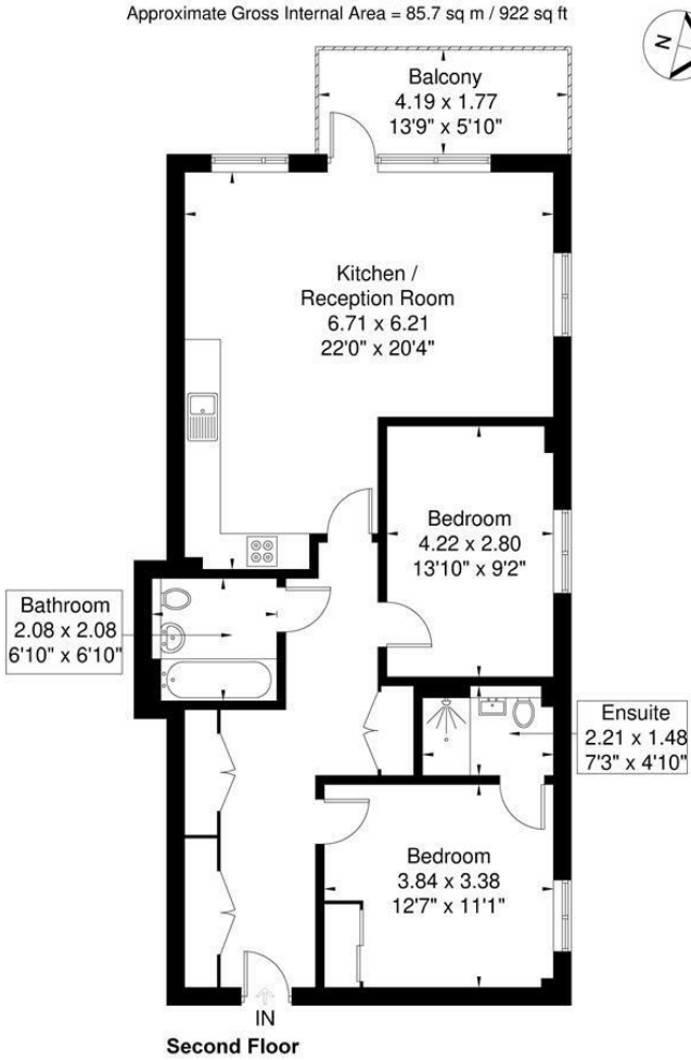
Munster Court Approximate Gross Internal Area = 85.7 sq m / 922 sq ft
