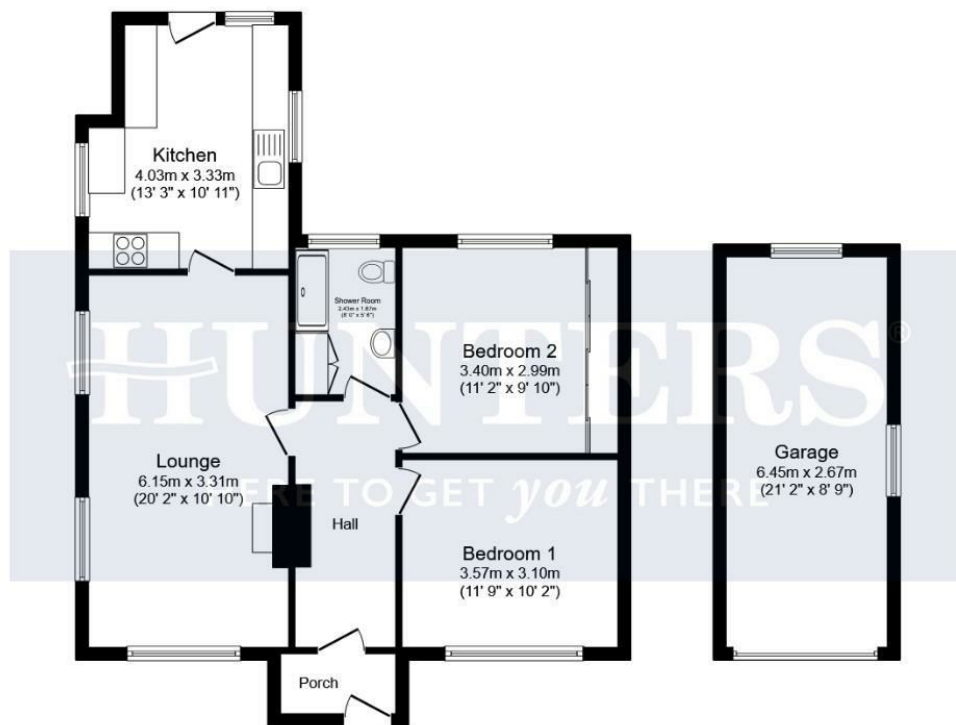
Floor Plan
