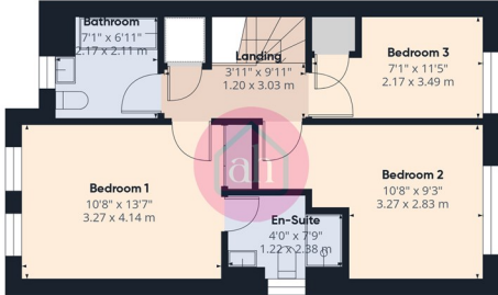
Floor 1 Building 1
