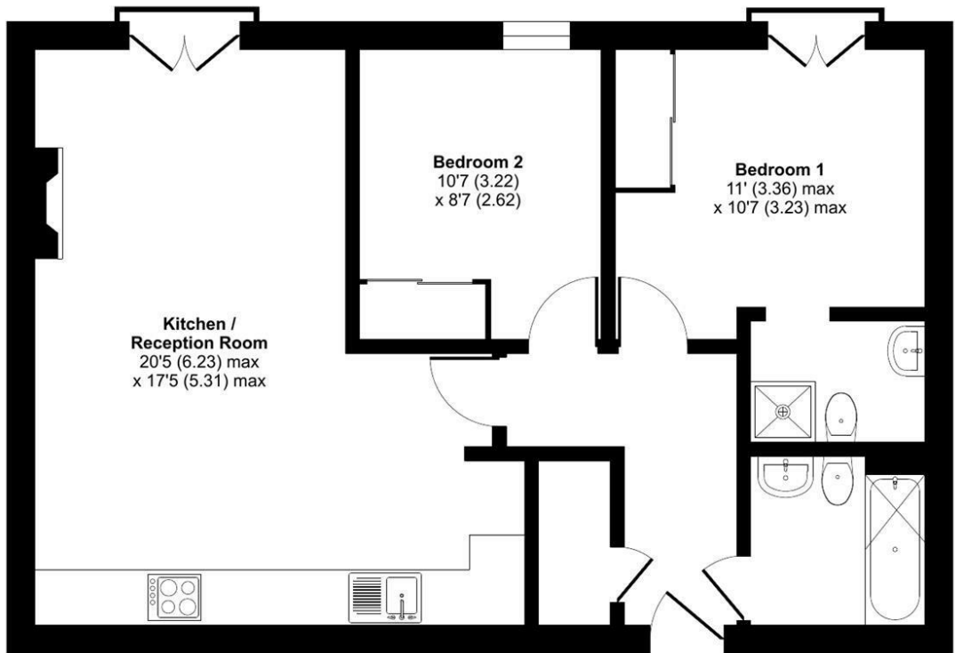
GROUND FLOOR
