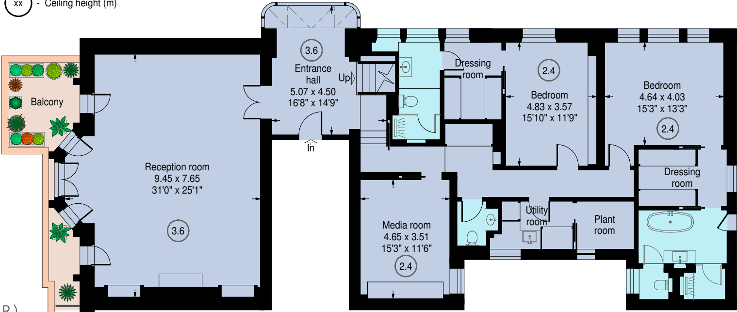
FIRST FLOOR (UPPER)
