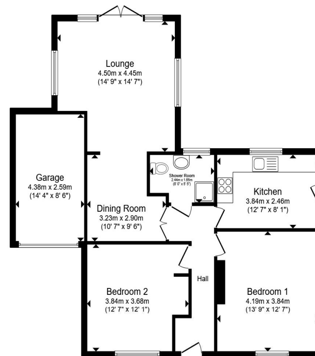
Floor Plan
