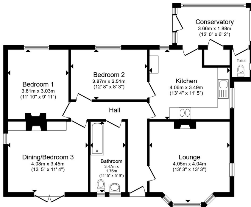
Floor Plan
