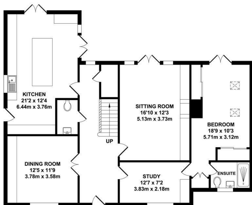
GROUND FLOOR APPROX. FLOOR AREA 1116 SQ.FT. (103.67 SQ.M.)
