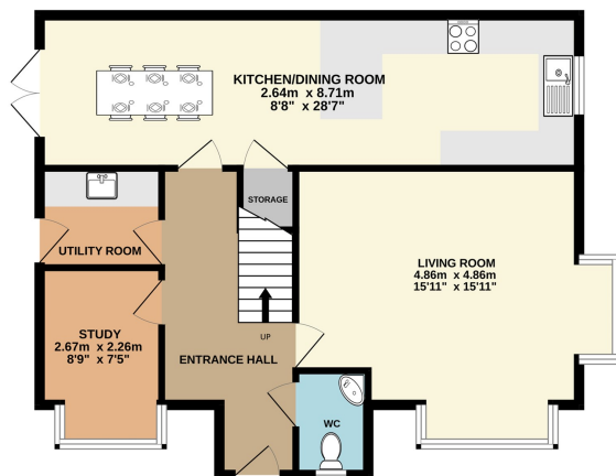
GROUND FLOOR 69.5 sq.m. (748 sq.ft.) approx.
