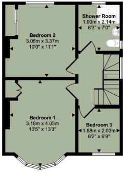
First Floor Approx 38 sq m / 408 sq ft
