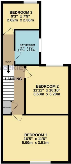
1ST FLOOR 525 sq. ft. (48.8 sq.m.) approx.
