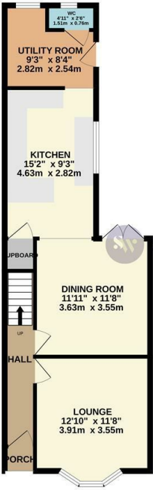
GROUND FLOOR 568 sq. ft. (52.8 sq.m.) approx.
