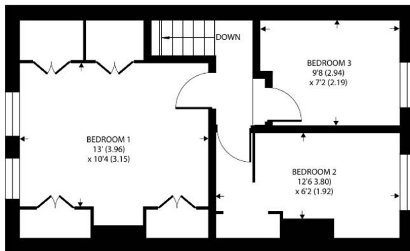
FIRST FLOOR
