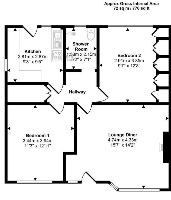
Ground Floor Approx 67 sq m / 724 sq ft
