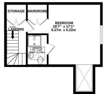
2ND FLOOR 343 sq.ft. (31.9 sq.m.) approx.
