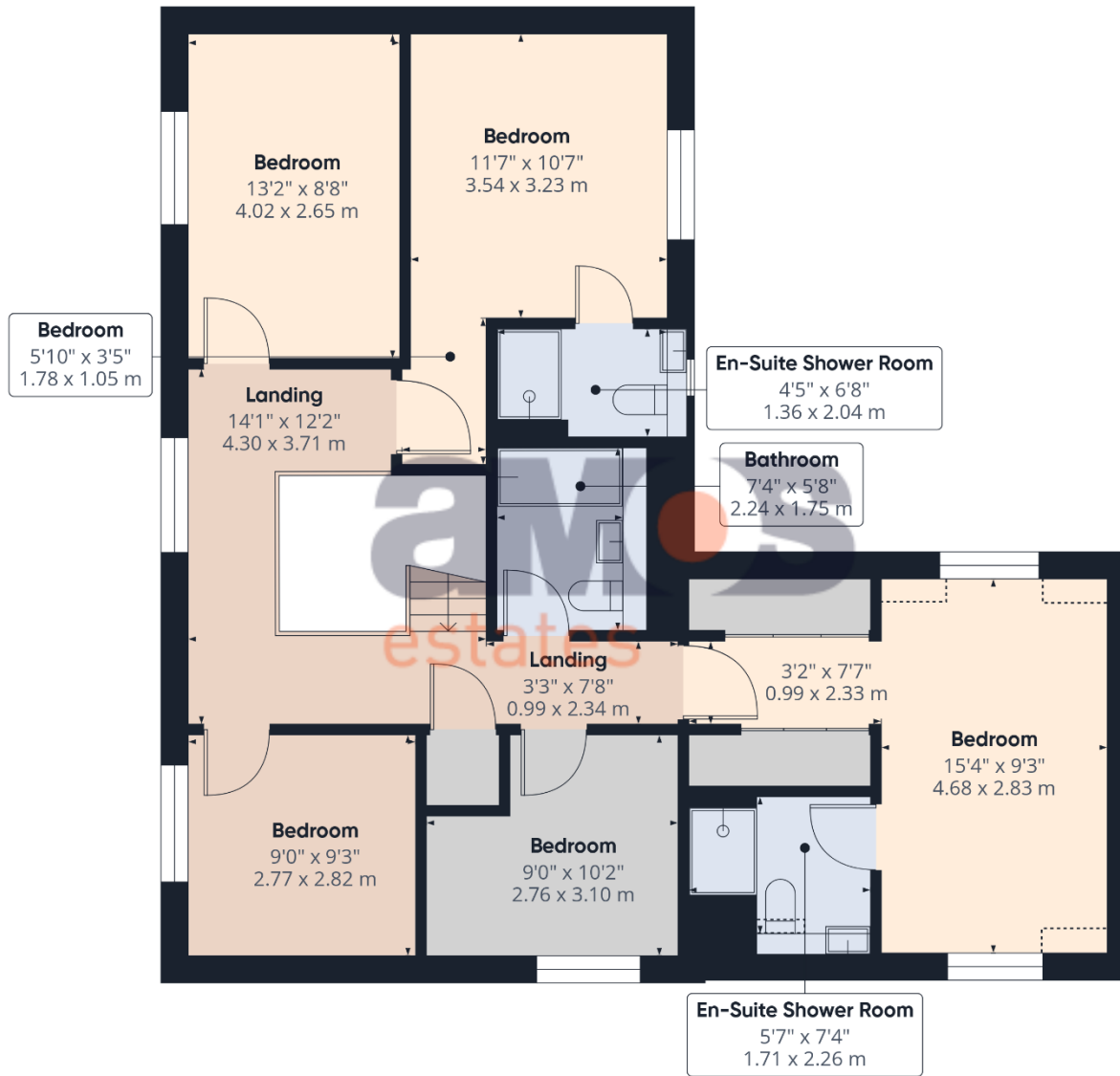
First Floor Building 1
