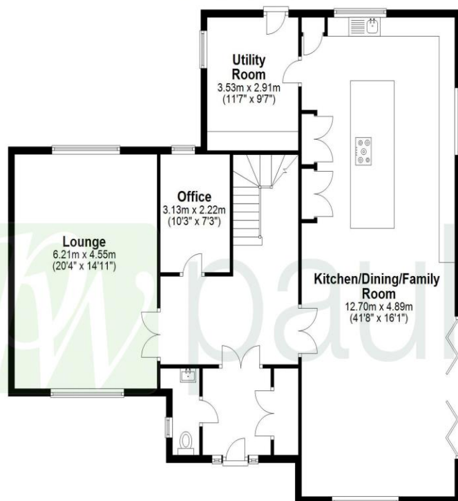
Ground Floor Approx. 136.7 sq. metres (1471.8 sq. feet)
