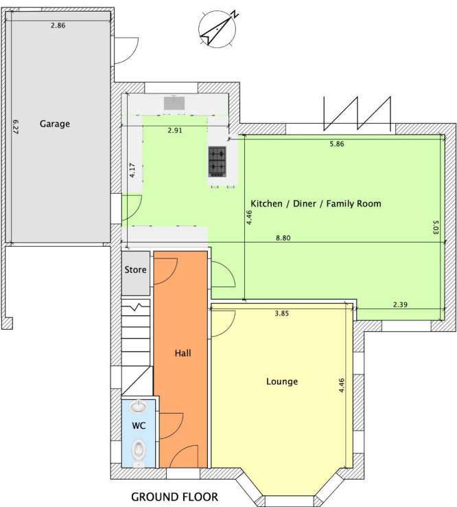
Indicative floor plans for illustration purposes only Approximate Gross Internal Floor Area 1,750 ft2
