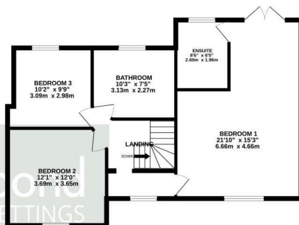
1ST FLOOR 744 sq.ft. (69.1 sq.m.) approx.
