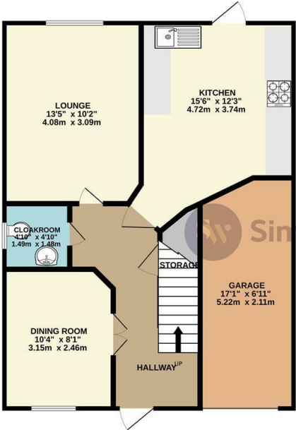
GROUND FLOOR 613 sq.ft. (57.0 sq.m.) approx.
