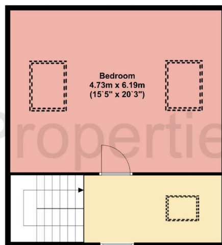
First Floor Approx 41.00 Sq meters (441.00 Sq feet).
