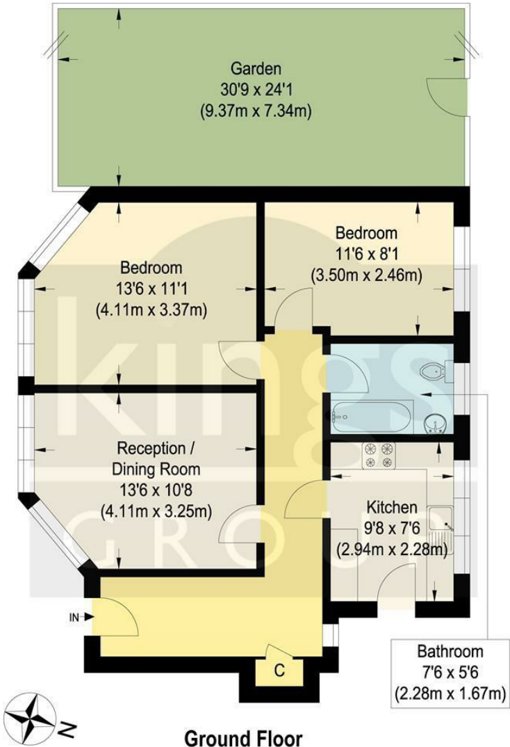
Ground Floor Beresford Gardens Approximate Gross Internal Floor Area : 59.20 sq m / 637.22 sq ft Illustration for identification purposes only, measurements are approximate, not to scale.
