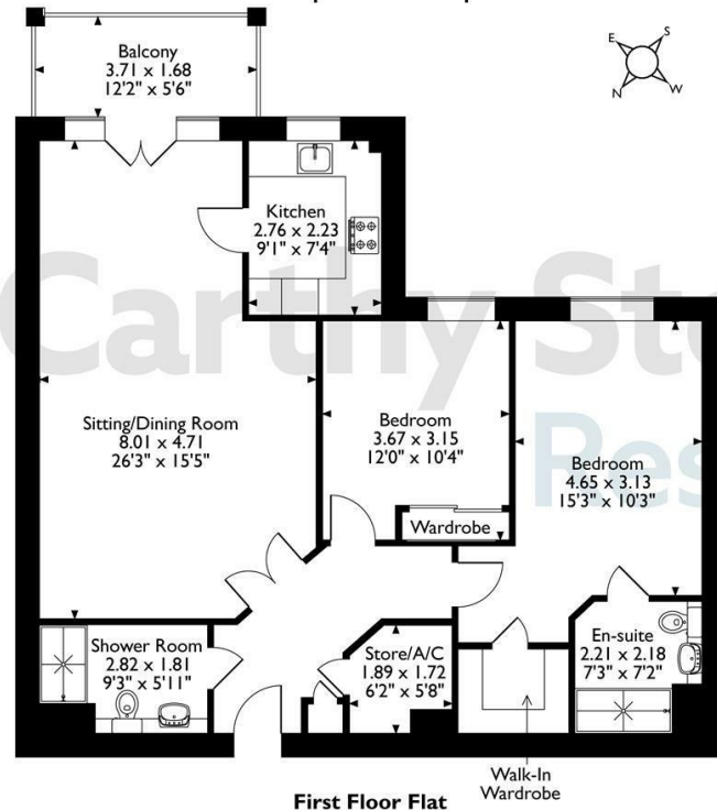
First Floor Flat The position & size of doors, windows, appliances and other features are approximate only. © ehoush. Unauthorised reproduction prohibited. Drawing ref. dig/8681987/DST.
