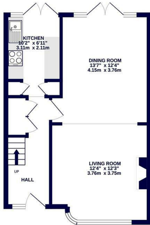
GROUND FLOOR 444 sq.ft. (41.2 sq.m.) approx.
