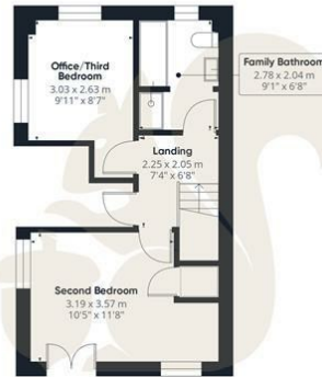
Floor 1 Building 1
