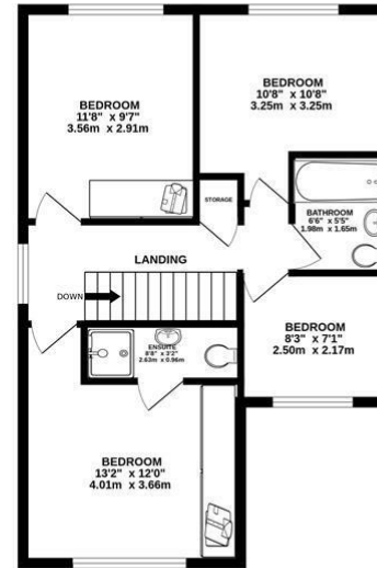
TOTAL FLOOR AREA: 1488 sq.ft. (138.3 sq.m.) approx. Measurements are approximate. Not to scale. Illustrative purposes only Made with Metropix ©2026
