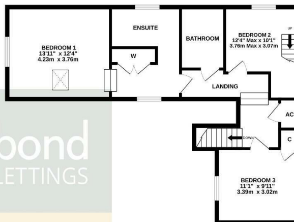
1ST FLOOR 668 sq.ft. (62.1 sq.m.) approx.
