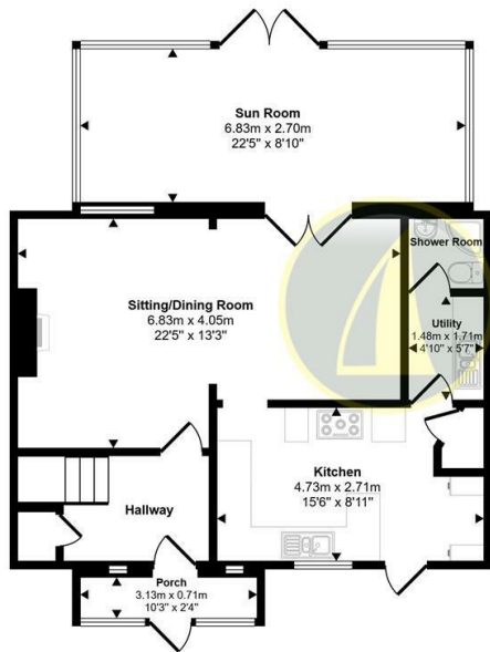
Ground Floor Approx 74 sq m / 796 sq ft
