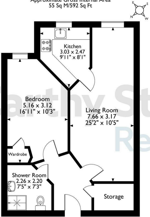
Third Floor
