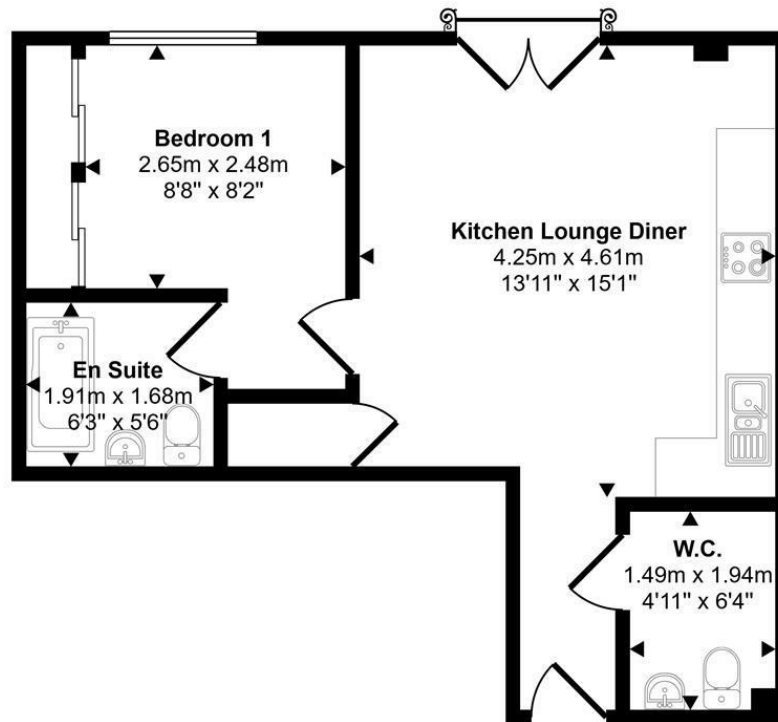
Floorplan
