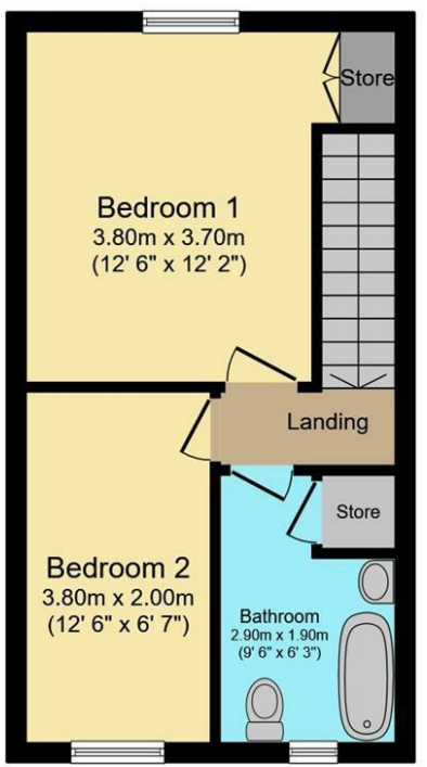
First Floor Floor area 30.8 sq.m. (331 sq.ft.)
