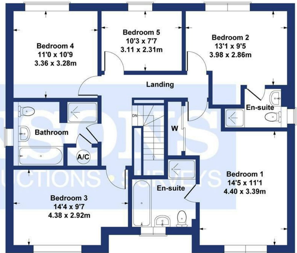
FIRST FLOOR
