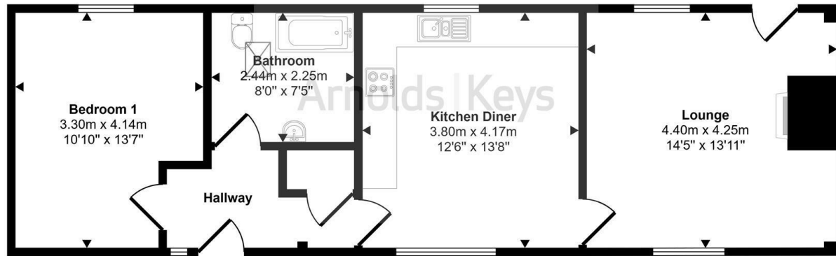
Floorplan
