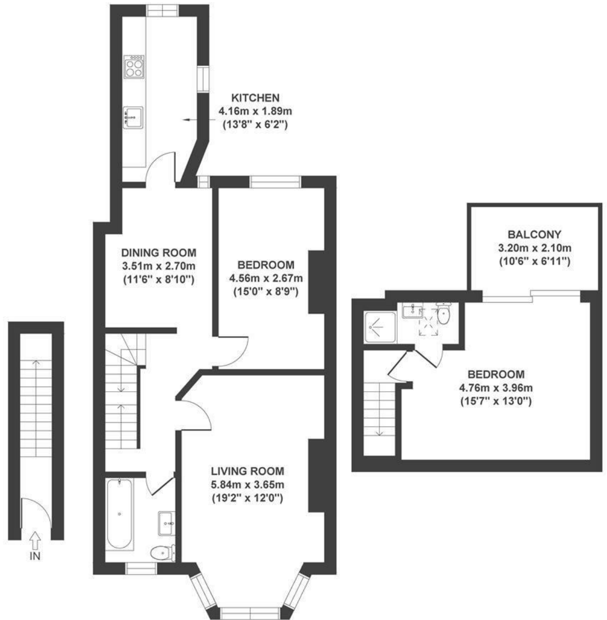
GROUND FLOOR
