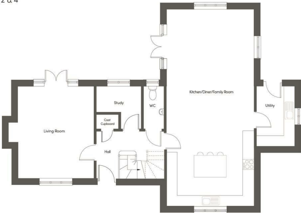
The Hampton Ground Floor Plots 2 & 4
