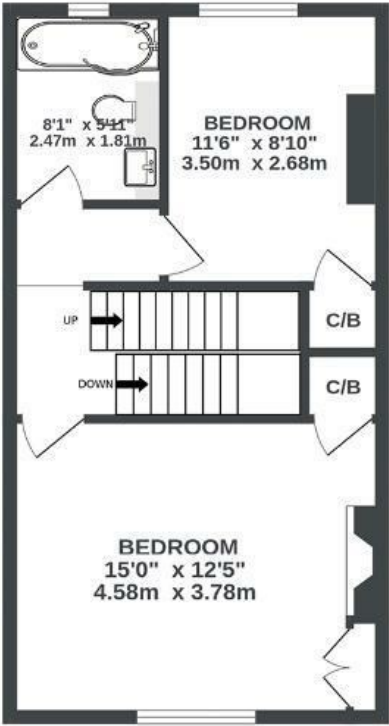
1ST FLOOR 432 sq.ft. (40.1 sq.m.) approx.
