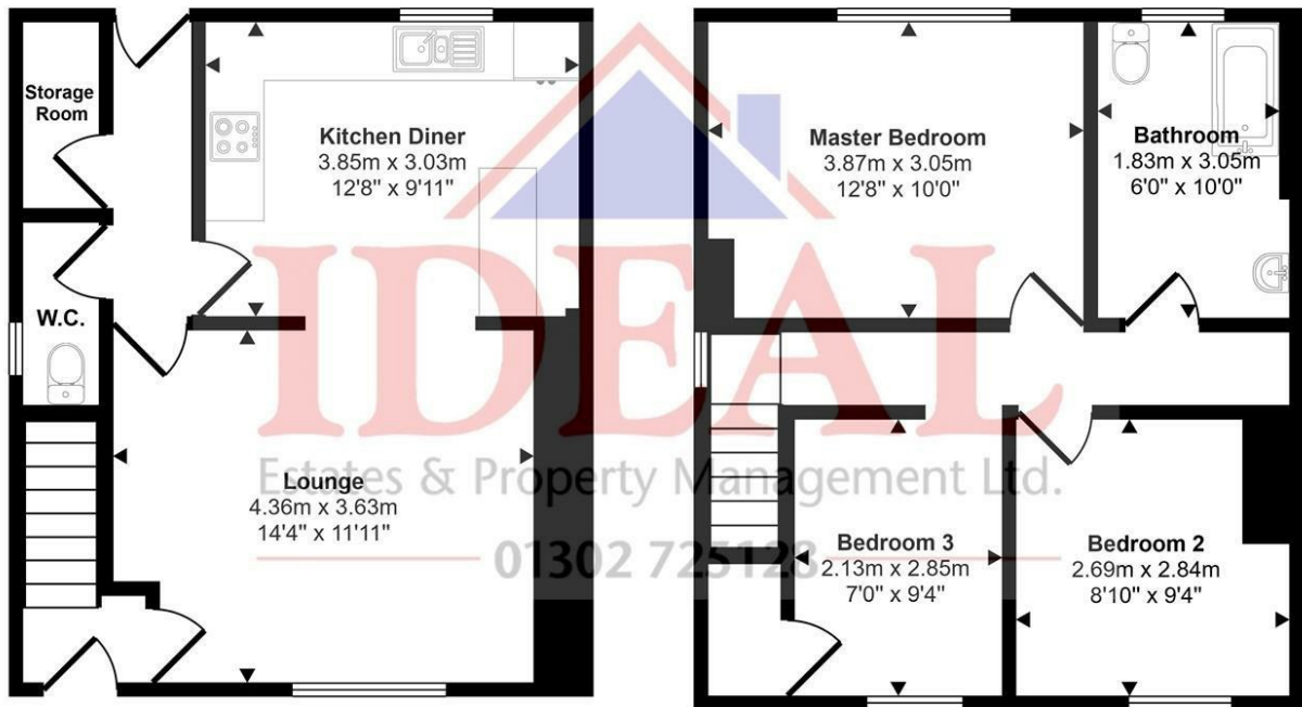
Ground Floor Approx 39 sq m / 423 sq ft
