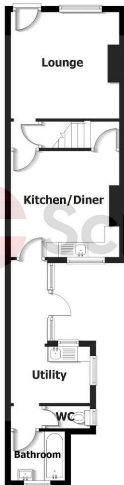
Ground Floor
