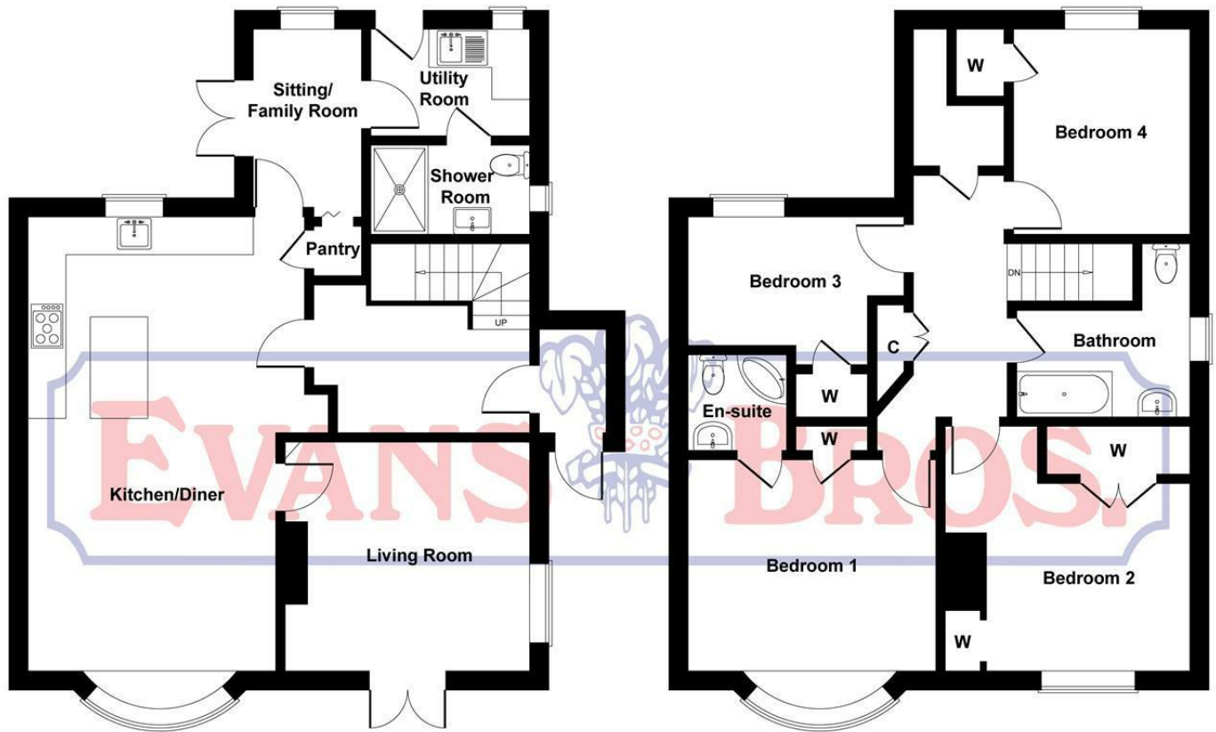
GROUND FLOOR
