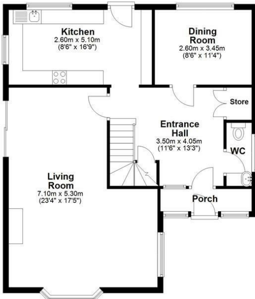
Ground Floor Approx. 75.9 sq. metres (817.4 sq. feet)
