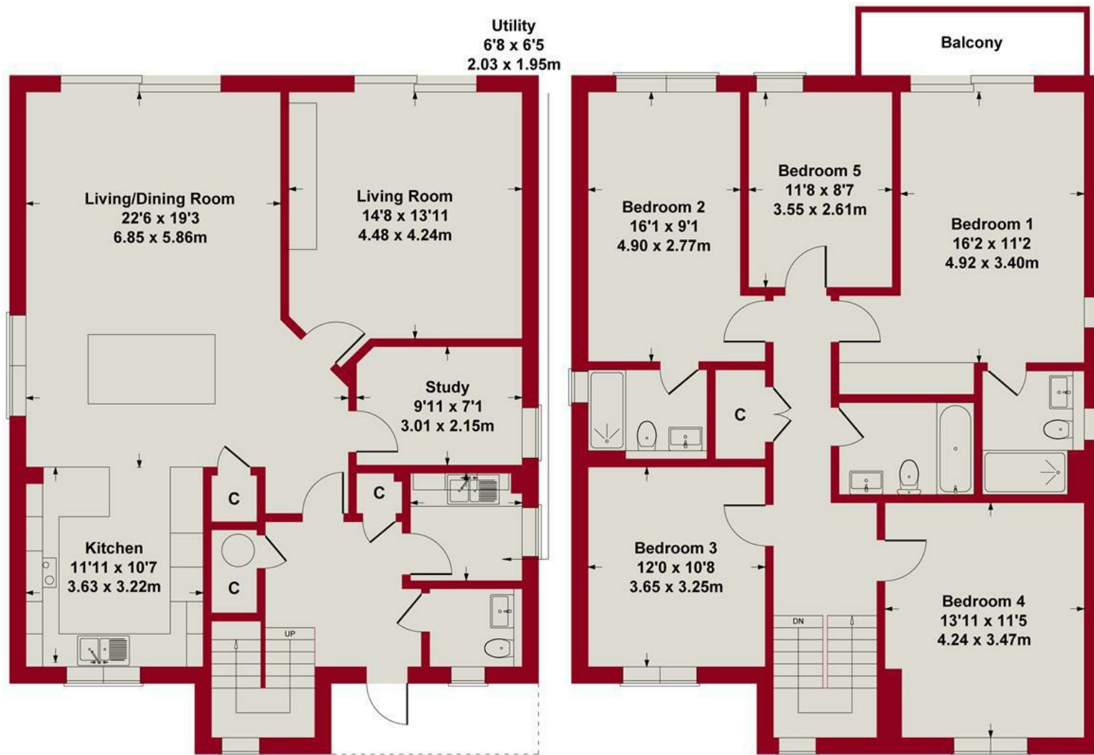
GROUND FLOOR
