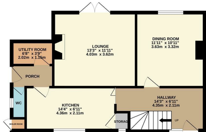
GROUND FLOOR 537 sq.ft. (49.9 sq.m.) approx.
