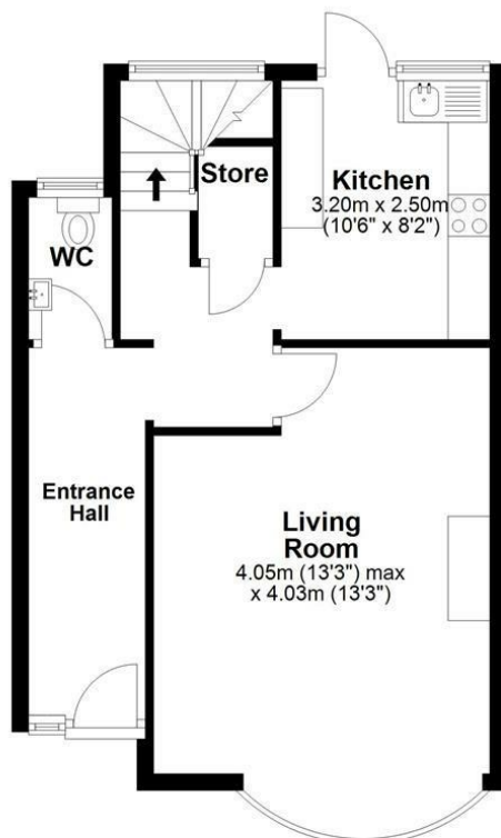
Ground Floor Approx. 44.4 sq. metres (477.5 sq. feet)
